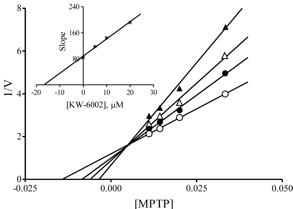
Figure 8. Lineweaver–Burke plots of the rates of the mouse brain MAO-B catalyzed oxidation of MPTP carried out in the absence (open circles) and presence of various concentrations of KW-6002 (filled circles, 5 \mu\text{M} ; open triangles, 10 \mu\text{M} ; filled triangles, 20 \mu\text{M} ). The secondary plot of the slopes of the Lineweaver–Burke plots versus the concentrations of KW-6002 (inset) gave a K_i value of 17 \mu\text{M} .
