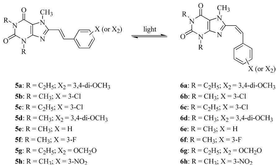
Figure 5. Photo-induced isomerization of ( E )-8-styryl-7-methylxanthinyl derivatives.
