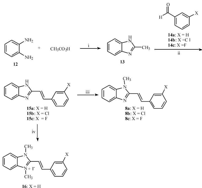
Figure 4. Synthetic pathway to substituted ( E )-2-styrylbenzimidazolyl analogues 8a–8c and 16 : (i) 4 N HCl, reflux 1 h; (ii) 180 °C, 24 h; (iii) \text{CH}_3\text{I} (1 equiv), \text{K}_2\text{CO}_3 , DMF, rt; (iv) \text{CH}_3\text{I} (2 equiv), \text{K}_2\text{CO}_3 , DMF, 100 °C.
