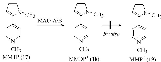
Figure 7. The MAO catalyzed oxidation of MMTP ( 17 ) to the corresponding dihydropyridinium species ( 18 ). The further oxidation of 18 to the pyridinium species 19 is not observed.
