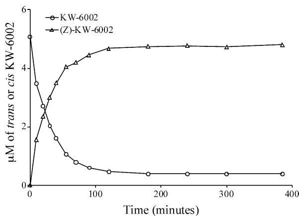
Figure 6. A graphical representation of the isomerization of KW-6002 (circles) to its corresponding cis isomer (triangles) when a 5- \mu M solution was exposed to light for various periods of time.
