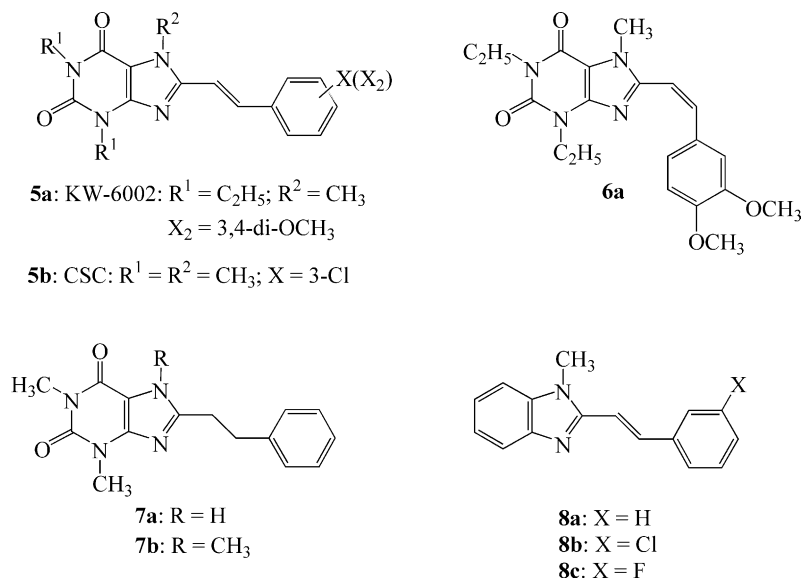
Figure 2. Structures of compounds discussed in the text.
