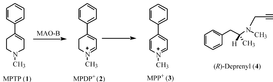
Figure 1. The MAO-B dependent bioactivation pathway for MPTP ( 1 ) via MPDP + ( 2 ) to MPP + ( 3 ) and the structure of the MAO-B inactivator ( R )-deprenyl ( 4 ).
